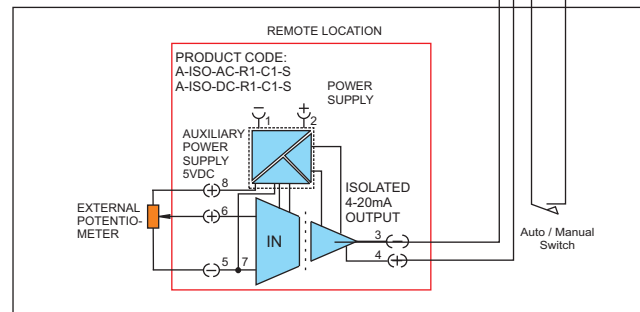
SCHEMATIC AND APPLICATION DIAGRAM: DC Current Isolator and Isolating Resistance to Current Converter
