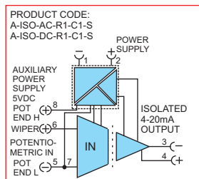
SCHEMATIC AND APPLICATION DIAGRAM: DC Current Isolator and Isolating Resistance to Current Converter
