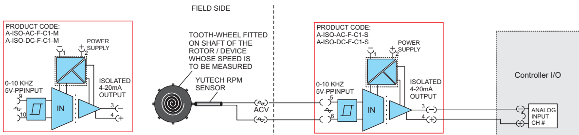
SCHEMATIC AND APPLICATION DIAGRAM: Isolating AC Signal Converter – Frequency (0-10KHz @ 5VPP), to Current (4 – 20 mA), VDC / VAC PS
