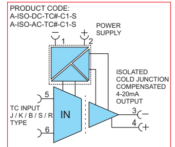
SCHEMATIC AND APPLICATION DIAGRAM: Isolating Temperature Transmitters - Input: 2/3W RTD PT-100, 4W RTD PT-100, 4W RTD PT-1000, TC, Output: 4-20mA
