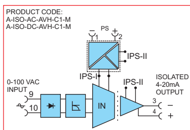
SCHEMATIC AND APPLICATION DIAGRAM: Isolating AC Signal Converter - High AC Voltage (0-100VAC) to standard DC Current (4 - 20 mA), VDC / VAC PS
